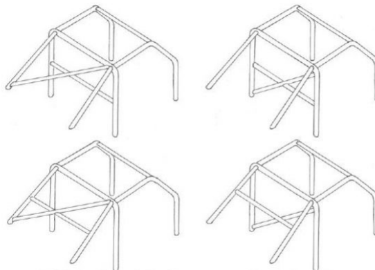
Diagram 5.4(c) – Principle Structure of a Safety Cage post 1 January 2013
