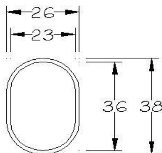
FRONT & REAR HOUSING
