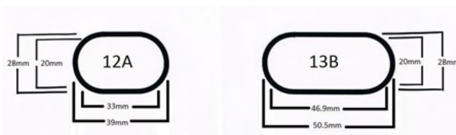
Drawing 4.3E: 12A and 13B exhaust ports, nominal dimensions in mm. The dimension 33mm to 39mm, 20mm to 28mm, and 46.9mm to 50.5mm show the chamfer that exists from the apex seal sealing surface face in the housing to the aperture before stainless steel exhaust sleeve, which is to be no deeper than 2mm. NIMRRA template is available.
